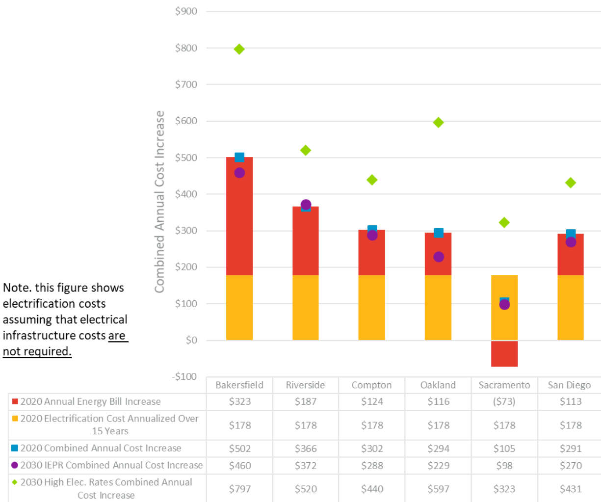
Figure 2-5. Electrification Cost Increases for Home Design A in 2020 and 2030 Scenarios (Assumes Electrical Infrastructure Upgrades are Not Required )
