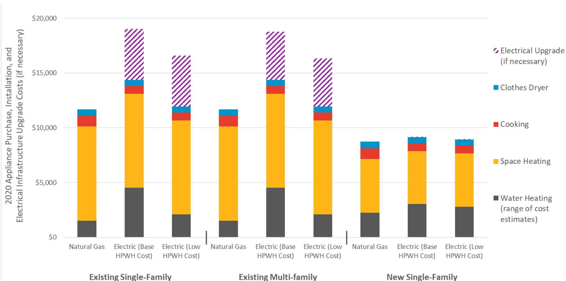
Figure 2-2. 2020 Total Appliance Purchase, Installation, and Electrical Infrastructure Upgrade Costs (if necessary), including Range of Water Heater Cost Estimates
