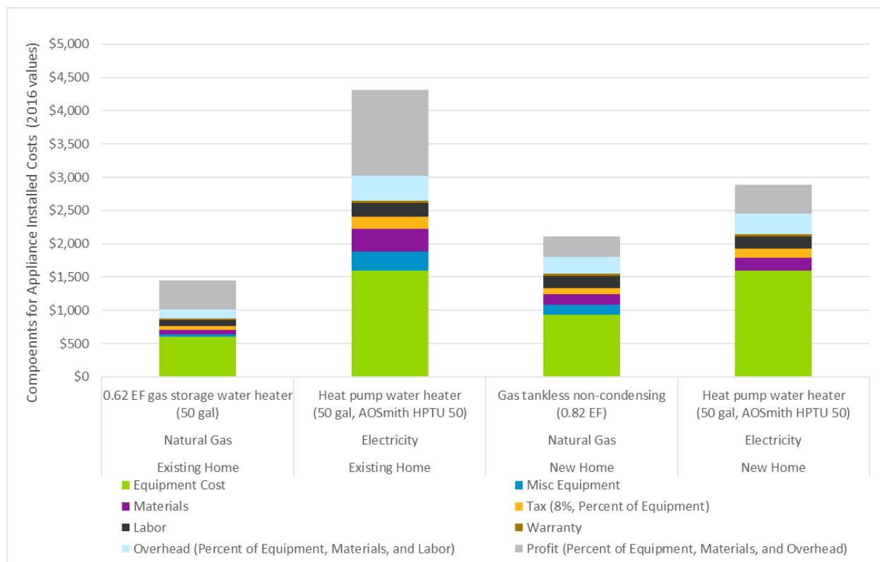
Figure A-1. Representative Buildup of Appliance Cost in Analysis (2016 values, unadjusted for future years)
